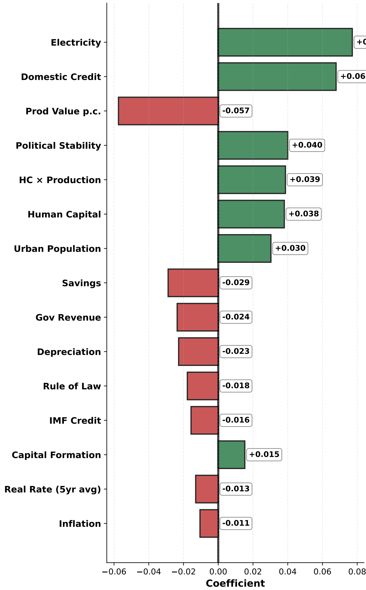
Ridge Train R 2 =0.783 Test R 2 =0.847 | 24 features
