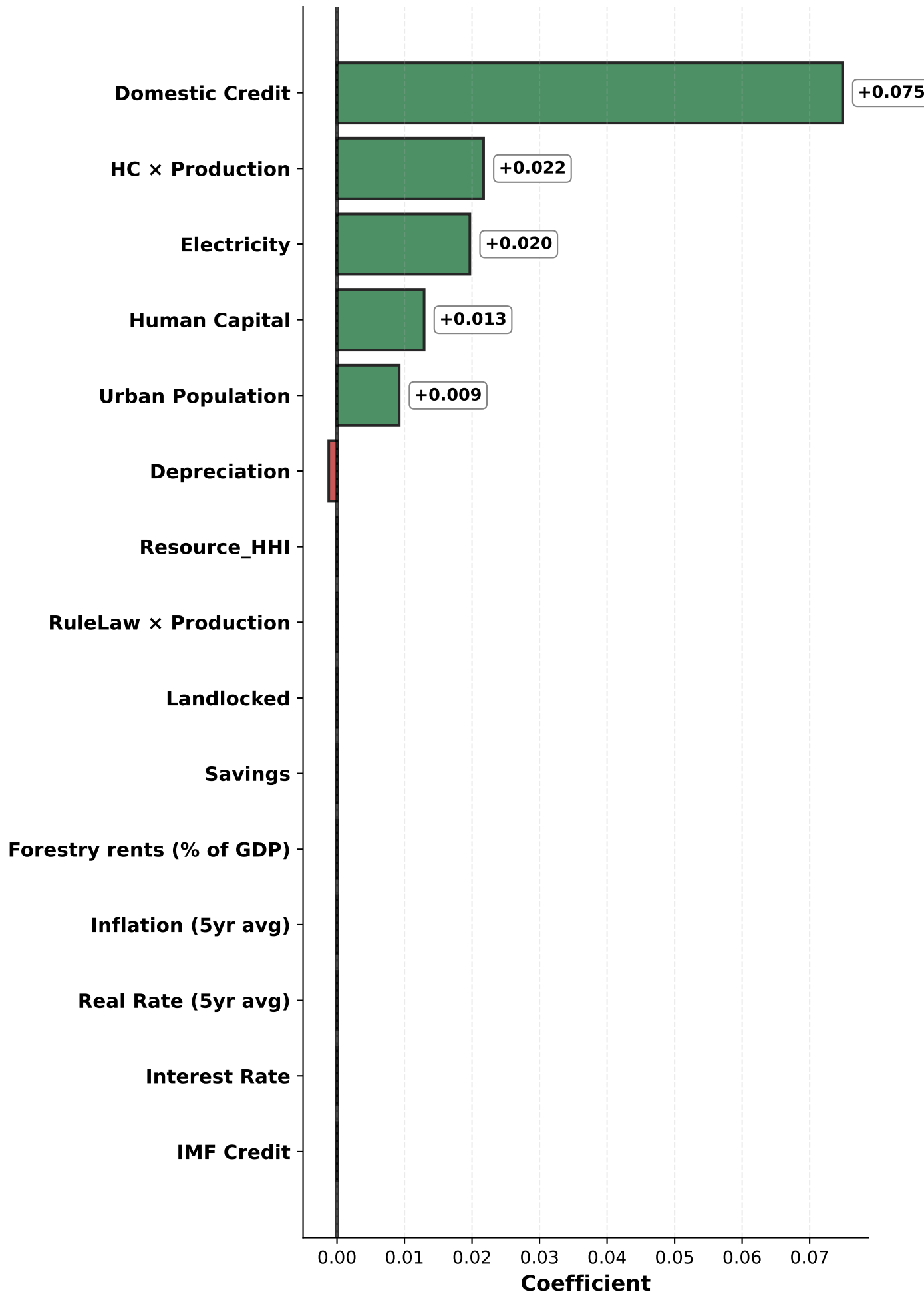
Elastic Net Train R 2 =0.770 Test R 2 =0.854 | 7 features
