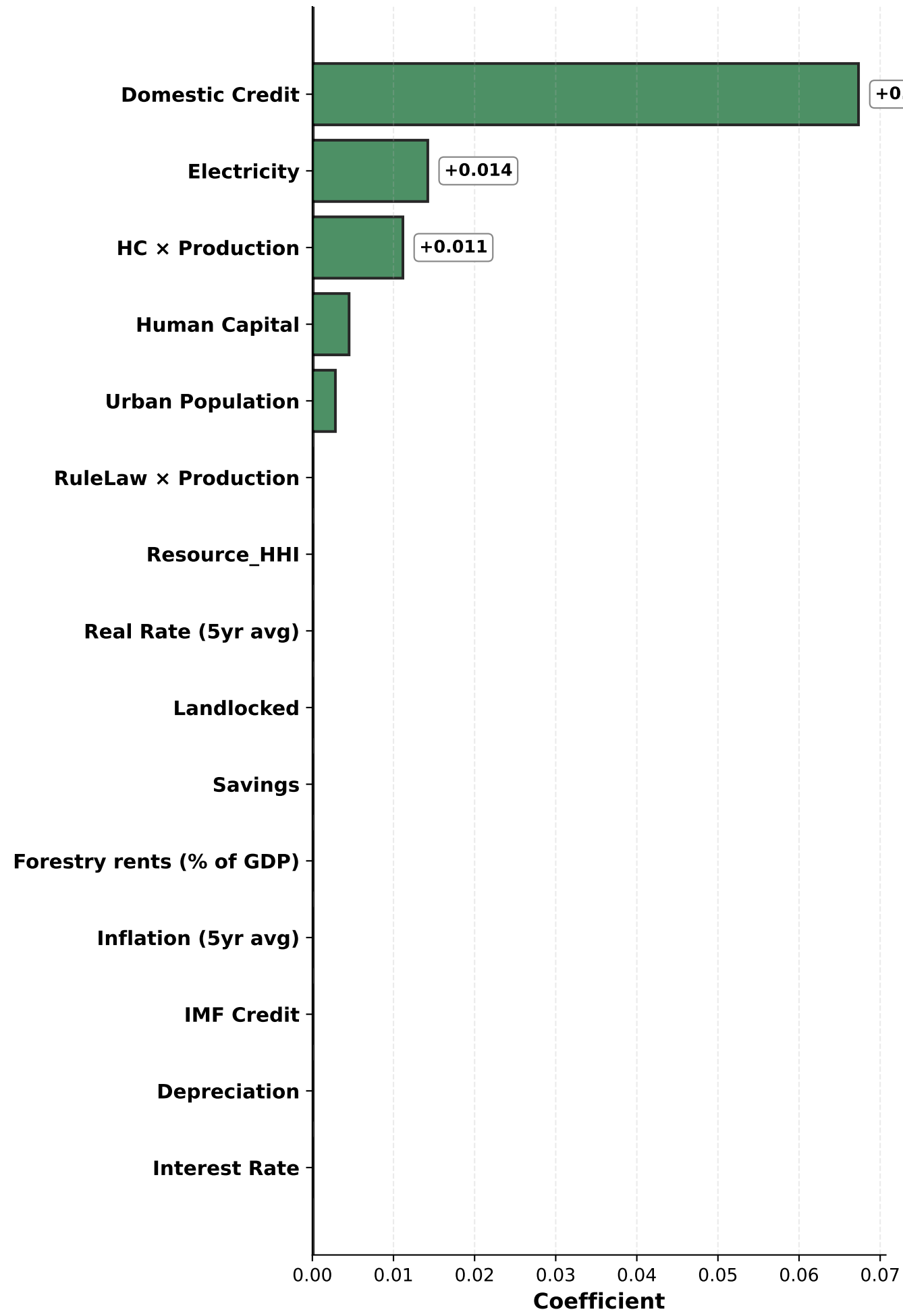
LASSO Train R 2 =0.769 Test R 2 =0.857 | 6 features
